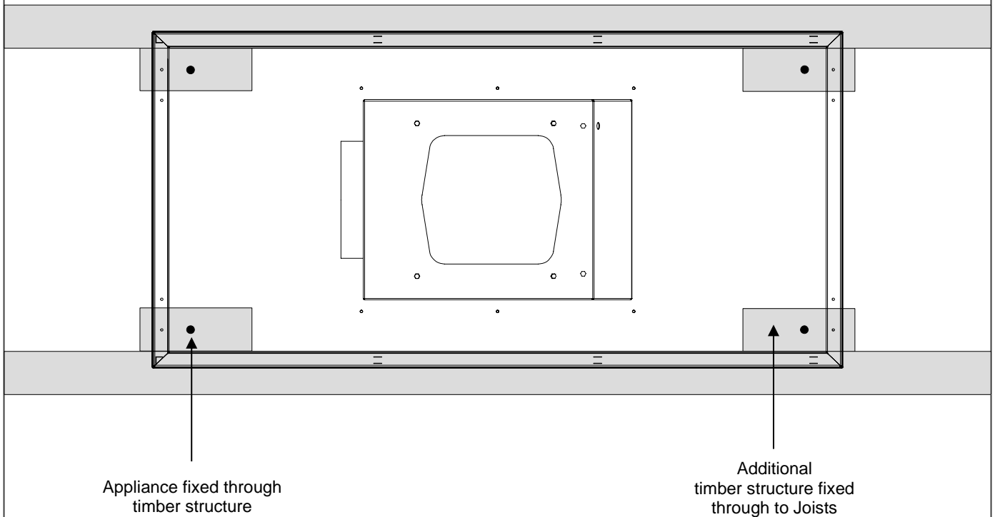
PLAN VIEW
