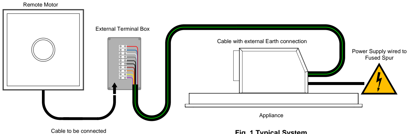
Fig. 1 Typical System
